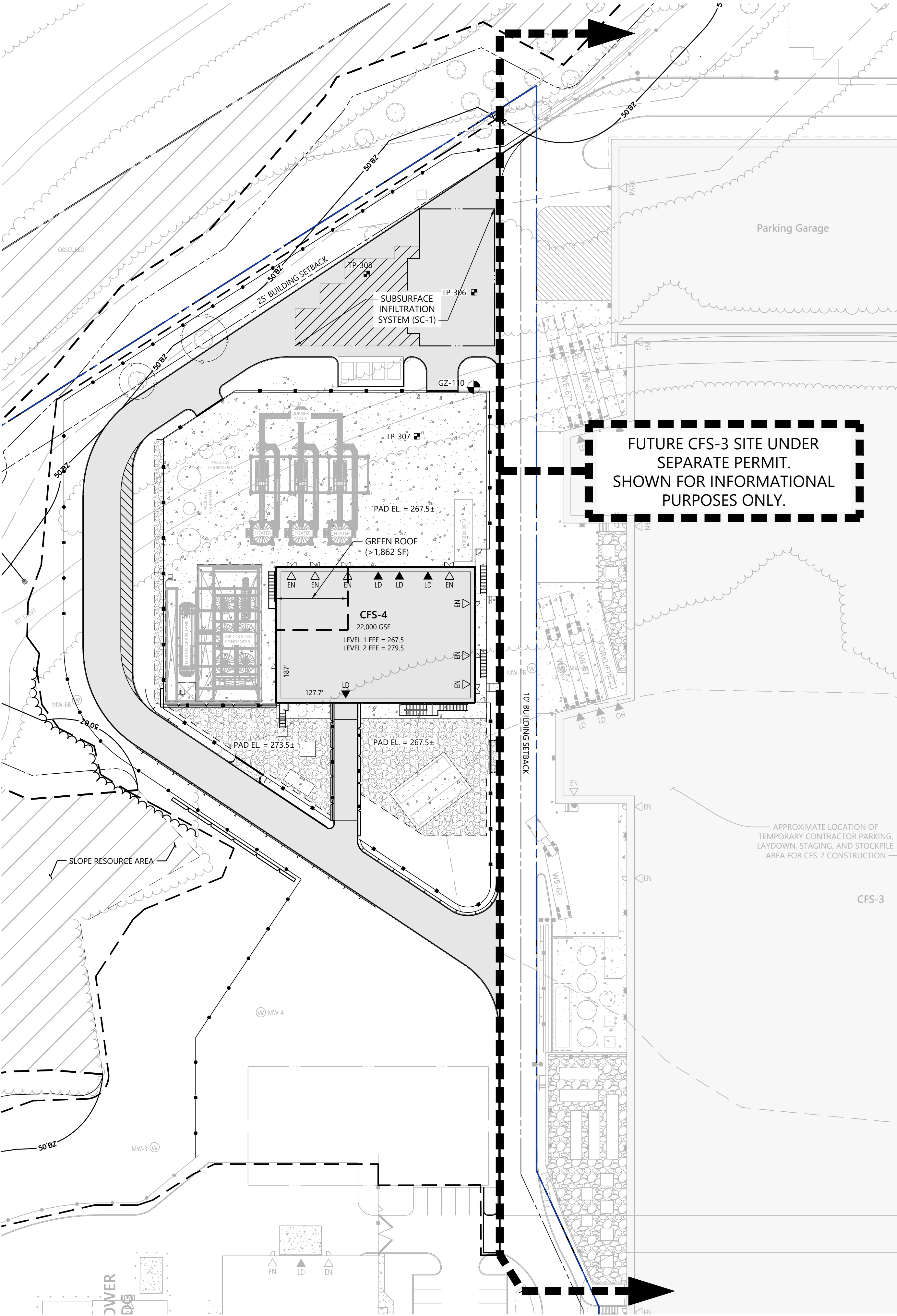
Revised Site Layout
